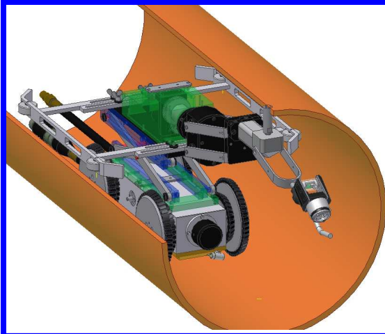
Cutter in 600mm Pipe
